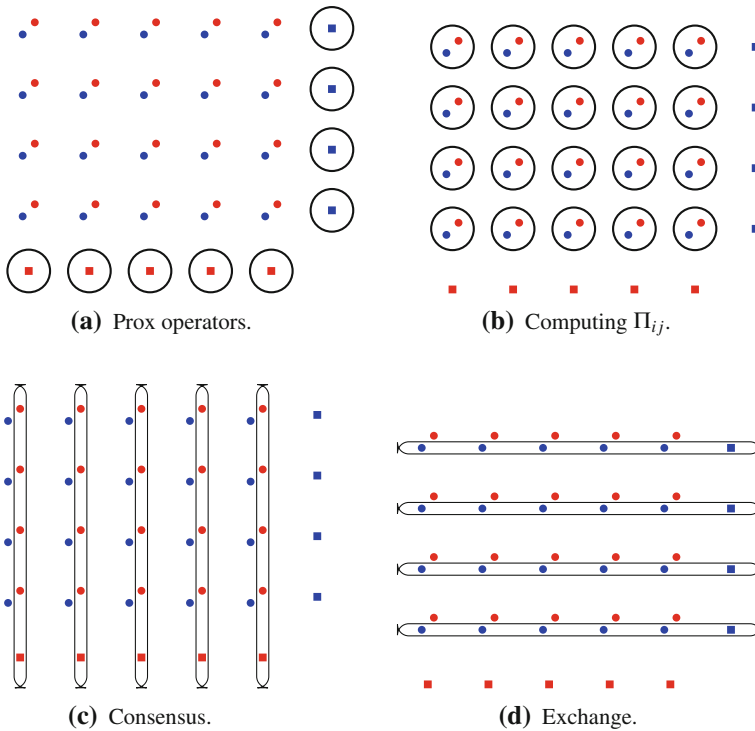
Fig. 1 Diagram of which nodes perform computations in which steps in each iteration. Red is x and blue is y ; the extra column on the right is for y_i and the extra row at the bottom is for x_j (square rather than circular dots). The only omitted step, the dual update, splits completely (color figure online)
