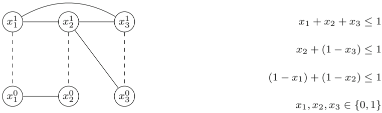
Fig. 2 Example of a conflict graph for three binary variables, where x_i^0 and x_i^1 indicate setting x_i to 0 and 1 respectively. On the right, a linear representation of the constraints from the conflict graph
