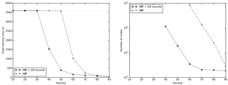
Fig. 6 Comparison in solving time and branch-and-bound tree size between applying and not applying DD bounds in independent set instances with 300 vertices. The gray dotted line on the left plot indicates the time limit of one hour. Unreported data on number of nodes corresponds to cases in which the time limit of one hour was hit on the majority of runs
