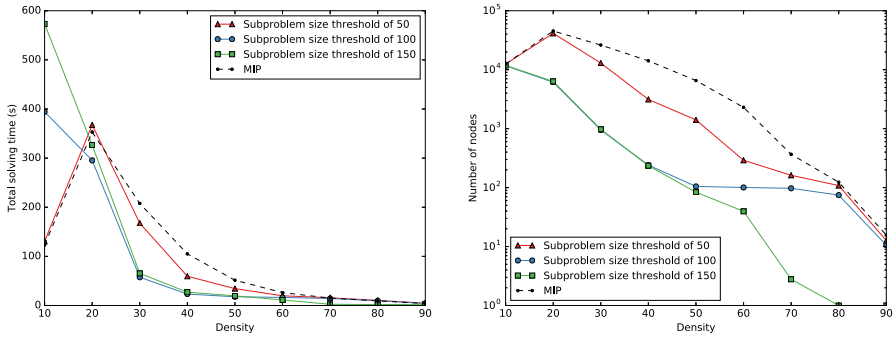
Fig. 7 Comparison of different subproblem size thresholds with 150 vertices
