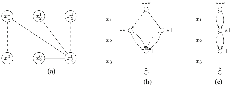
Fig. 3 a A conflict graph. b Decision diagram that would be obtained by using the DP formulation (IG) as is. The states are depicted as a sequence of symbols representing the domain of each completion variable following the order x_1, x_2, x_3 . The symbol is * if the domain is \{0, 1\} , 1 if it is \{1\} , and 0 if it is \{0\} . c Decision diagram obtained if we establish domain consistency at the root state, which is always reduced as proved in Theorem 1
