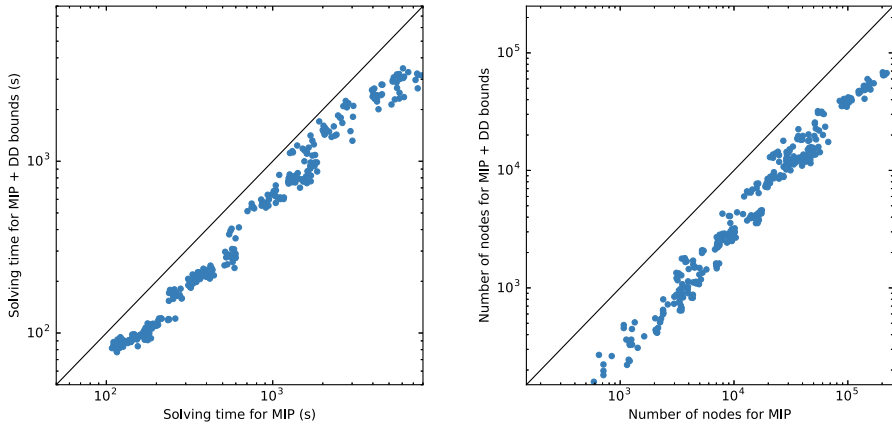
Fig. 11 Effect of using decision diagram bounds illustrated by individual independent set + knapsack instance. Each point is an instance + random seed and points below the diagonal line correspond to better performance than not using bounds
