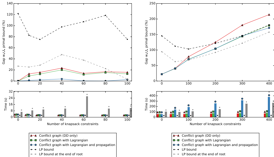
Fig. 9 The plot on the top illustrates a comparison of bound quality for independent set + knapsack constraints with 200 (left) and 1000 (right) variables, varying the number of knapsack constraints. The plot on the bottom represents the solve times to reach each bound. The quality of a bound D is represented by its gap (D - P)/P , where for n = 200 (left), P is the optimal value, and for n = 1000 (right), P is the best primal value given by the solver at its default settings after 10 min of solve time
