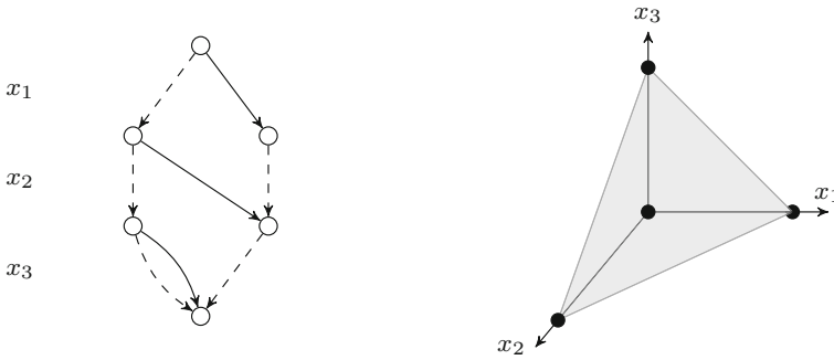
Fig. 1 On the left, a decision diagram that represents the set \{x \in \{0, 1\}^3 : x_1 + x_2 + x_3 \leq 1\} , pictured on the right. A dashed line indicates an arc with value zero, while a full line indicates an arc with value one. Each of the four paths from the root to the terminal nodes corresponds to a point in the set
