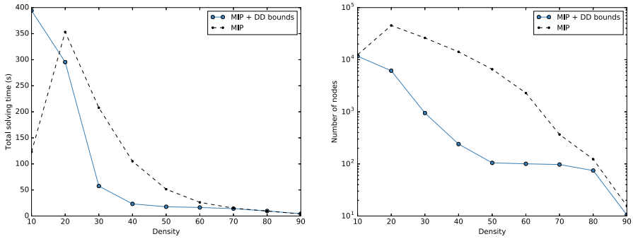
Fig. 5 Comparison in solving time and branch-and-bound tree size between applying and not applying DD bounds in independent set instances with 150 vertices. Results are averaged over solving 16 instances to optimality for each density parameter
