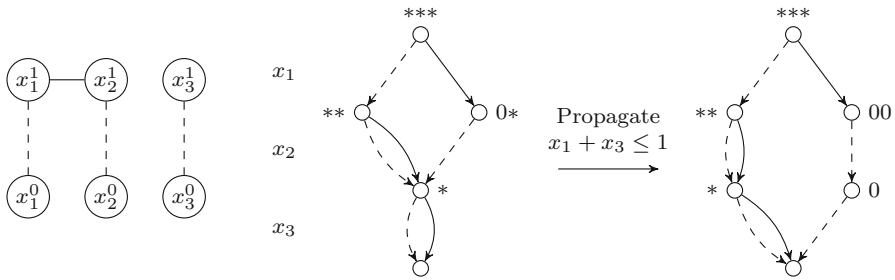
Fig. 4 An example in which propagation increases the size of the decision diagram in the context of conflict graphs
