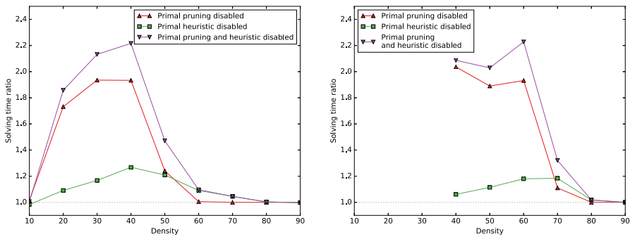
Fig. 8 Effect on solving time when disabling primal pruning and/or primal heuristic on instances of size 150 (left) and 300 (right). The vertical axis is the ratio t_d/T , where t_d is the time without a given feature and T is the time with all capabilities, and the horizontal axis is the density parameter of the set of instances. On the right, data points for densities below or equal 30 are omitted because the time limit is always hit
