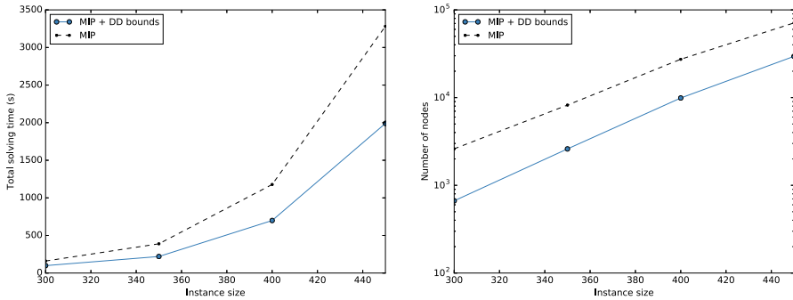
Fig. 10 Comparison in solving time and branch-and-bound tree size of the use of decision diagram bounds for independent set + knapsack instances
